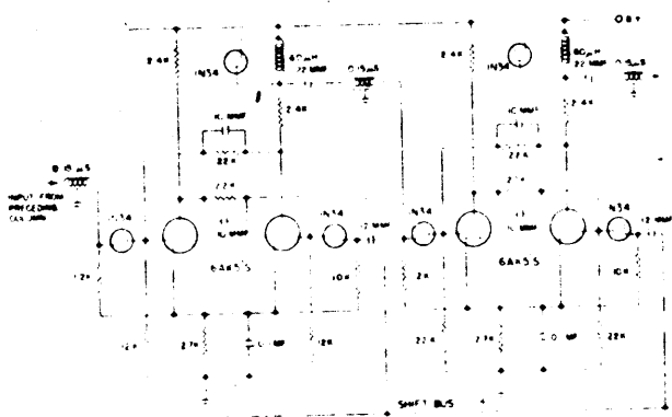
Fig. 10—Shift-register column.
