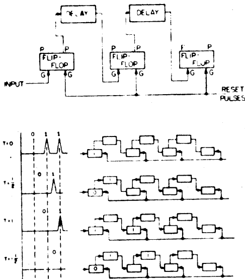
Fig. 9—Shift-register operation.
