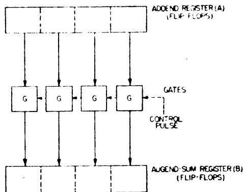
Fig. 8—Parallel-adder operation.
