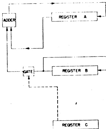
Fig. 7—Serial-adder operation.
